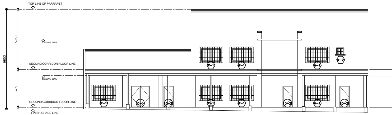
1 A-2 FRONT ELEVATION SCALE 1:100M
